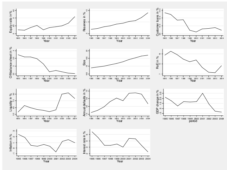
Figure 7: Evolution of bank-specific, distress, and macroeconomic covariates
