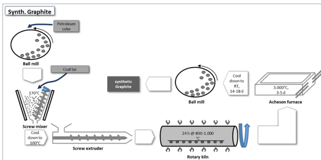
Figure 6: Overview of the synthetic graphite synthesis
