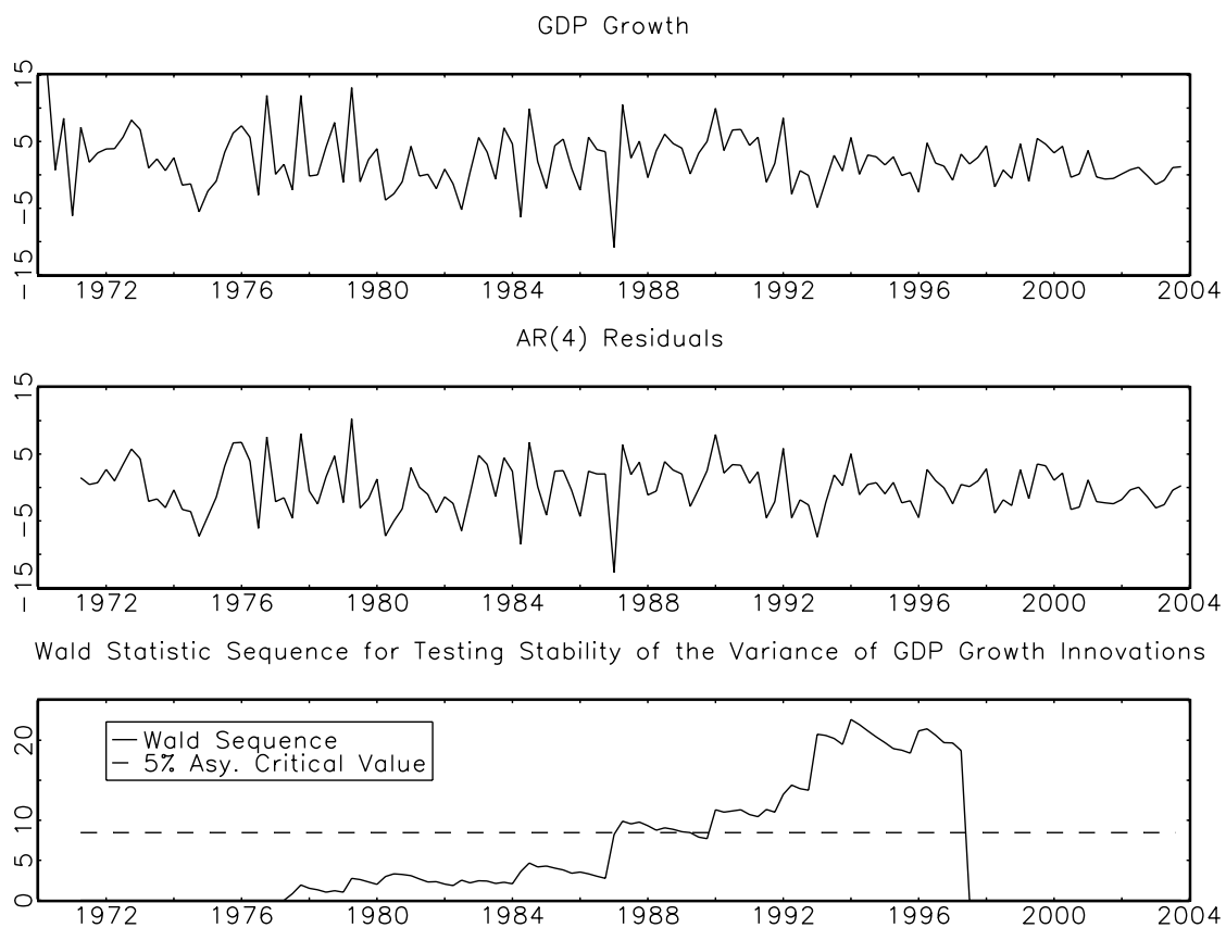
Fig. 1. German GDP growth from 1970:I to 2003:IV, measured in logged differences in quarterly GDP, annualized by multiplying by 400 (top panel); residuals from a AR(4) model (middle panel); sequence of the Wald statistics for testing for a break in the error variance of the AR(4) fitted to the GDP growth (bottom panel).
