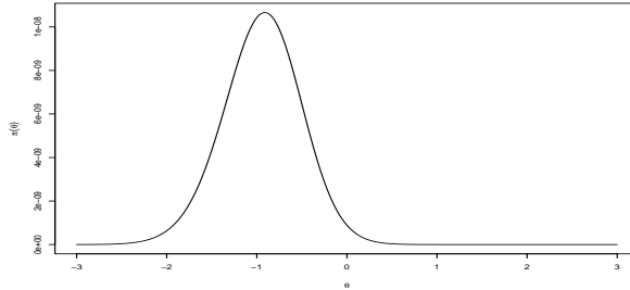
Fig. 1. Posterior density of \theta in the setting of Example 9 for n = 10 , with a simulated sample from \mathcal{T}(3, 0, 1) .
