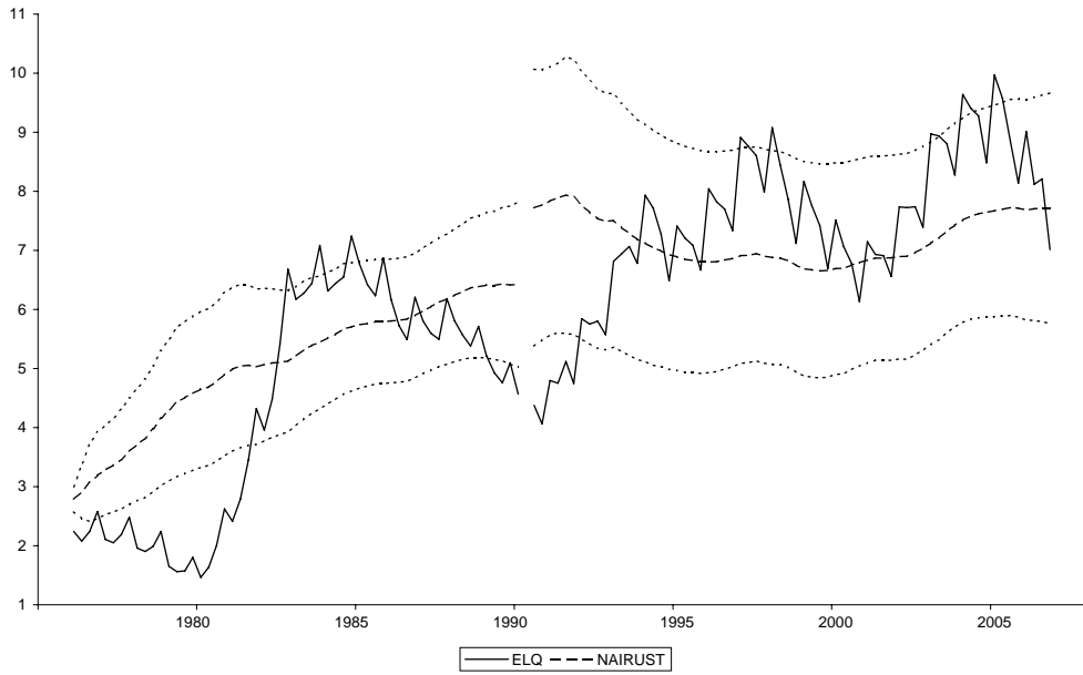
Figure 5: Nairu Estimates for Models 1–10 Nairu plus 90% confidence bands – Same Variance before/after Unification
