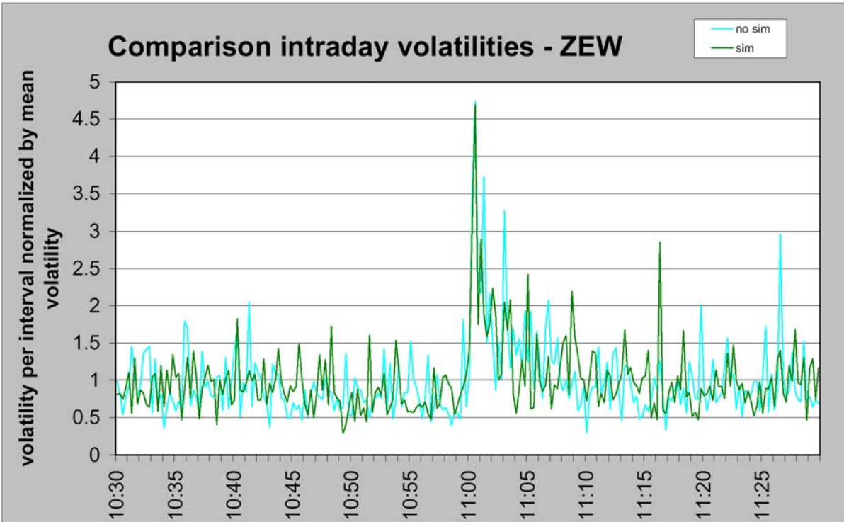
Figure 3: ZEW caused volatility \bar{V}_i/\bar{V} for 15-second intervals from 10:30 to 11:30
