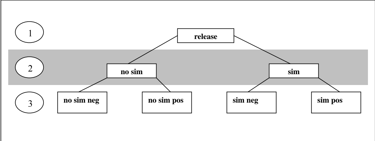
Figure 1: Design of estimation levels based on subsets of release days
