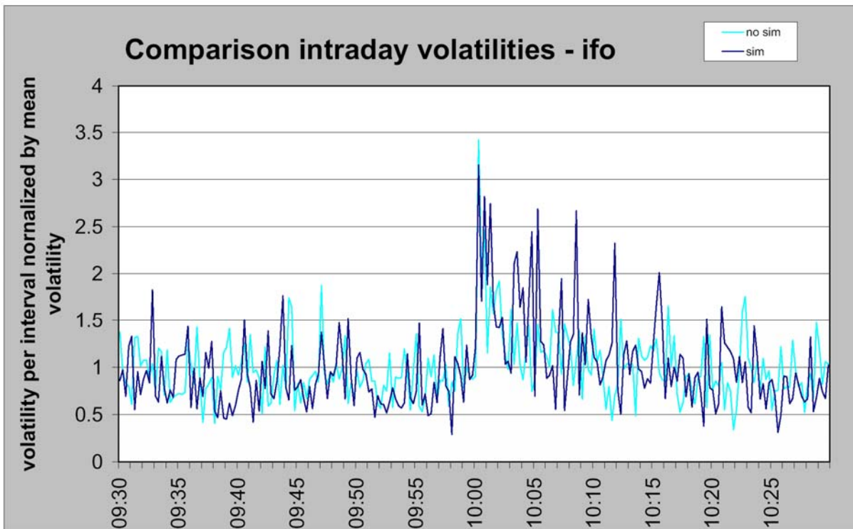
Figure 2: ifo caused volatility \bar{V}_i/\bar{V} for 15-second intervals from 09:30 to 10:30
