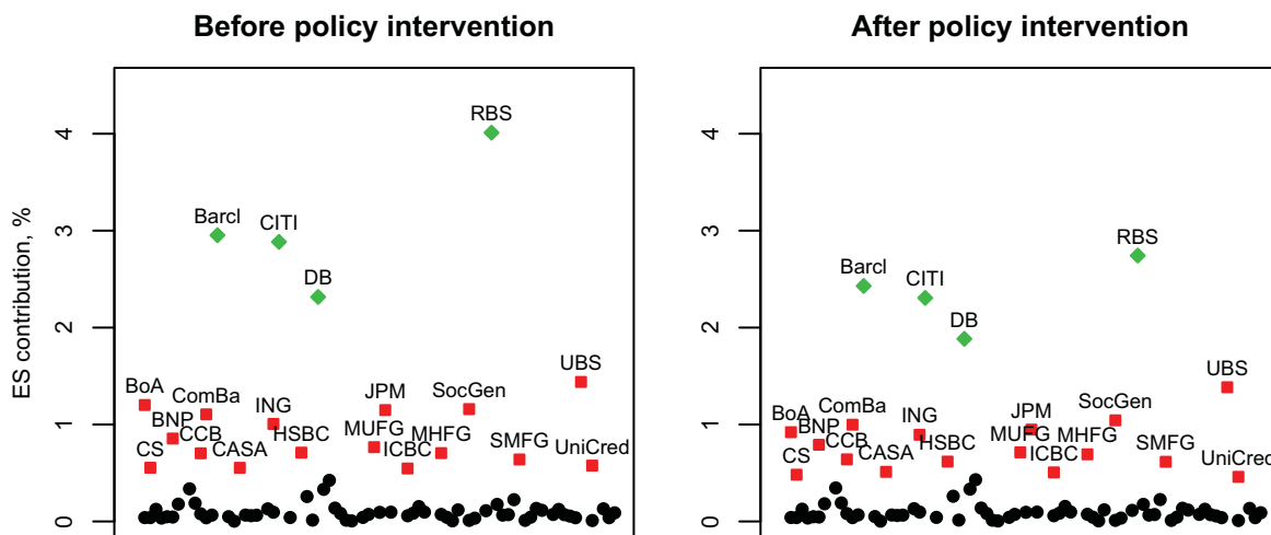
Figure 10: The landscape of systemically important banks before and after the policy intervention. 3 groups of banks have been identified by the k -means clustering method according to their contributions to the portfolio ES in January 2009. The banks are on the x-axis.
