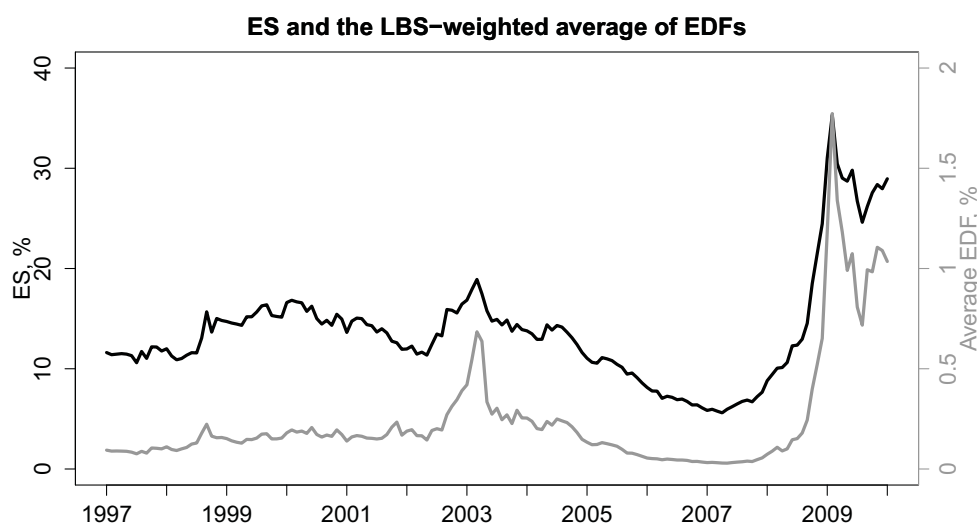
Figure 7: Evolution of the portfolio expected shortfall (ES, black lines, left axes) expressed as a percentage of the total portfolio liabilities (LBS). Also plotted is the weighted average of EDFs (gray lines, right axes); the weights are the shares of individual banks in the total LBS.
