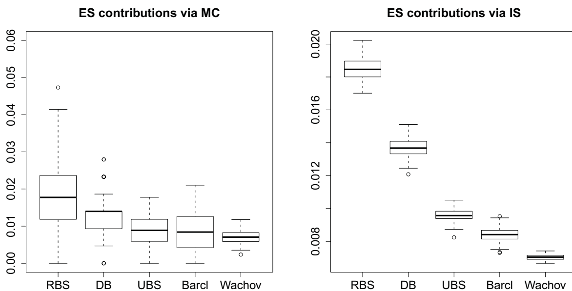
Figure 3: Comparison of the summary statistics for expected shortfall (ES) contributions in September 2008, estimated via Monte Carlo (MC) and importance sampling (IS). The box-and-whiskers plots are based on 100 independent scenarios. The five largest contributions are given as a fraction of the total liabilities of 84 banks in the portfolio.
