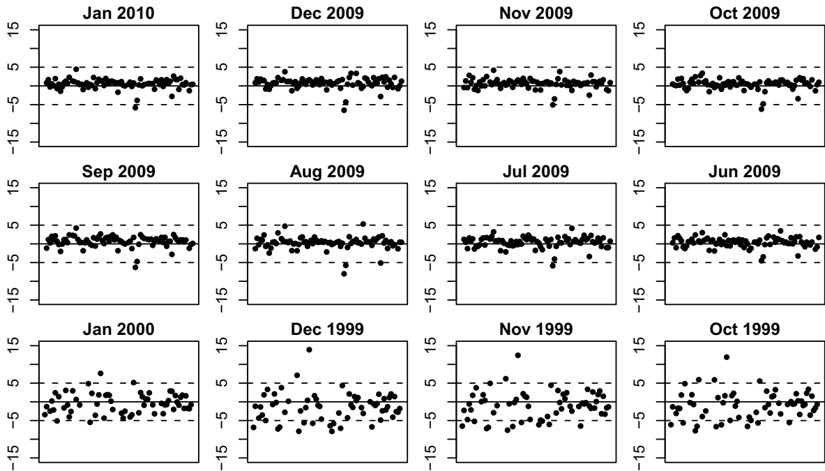
Figure 6: The relative difference (in percent) between the contributions to the expected shortfall estimated via importance sampling and those approximated analytically. The banks are on the x-axis.
