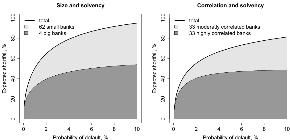
Figure 8: Systemic importance of two groups of banks with different sizes(left-hand plot) and different exposure to the single systematic factor (right-hand plot). Each of the two groups accounts for half of the total portfolio exposure.
