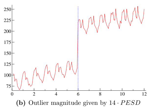
Figure B.5: Examples of series simulated with a level shift of two different magnitudes at 0.5 of the sample
