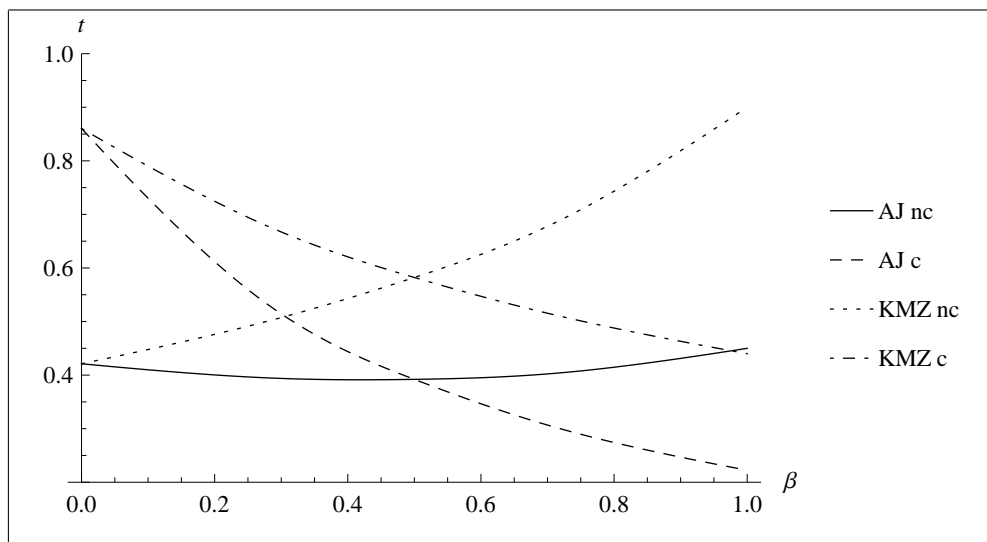
Figure 3: Optimal emissions tax - AJ and KMZ ( a = 20, e = 0.5, \gamma = 8 )
