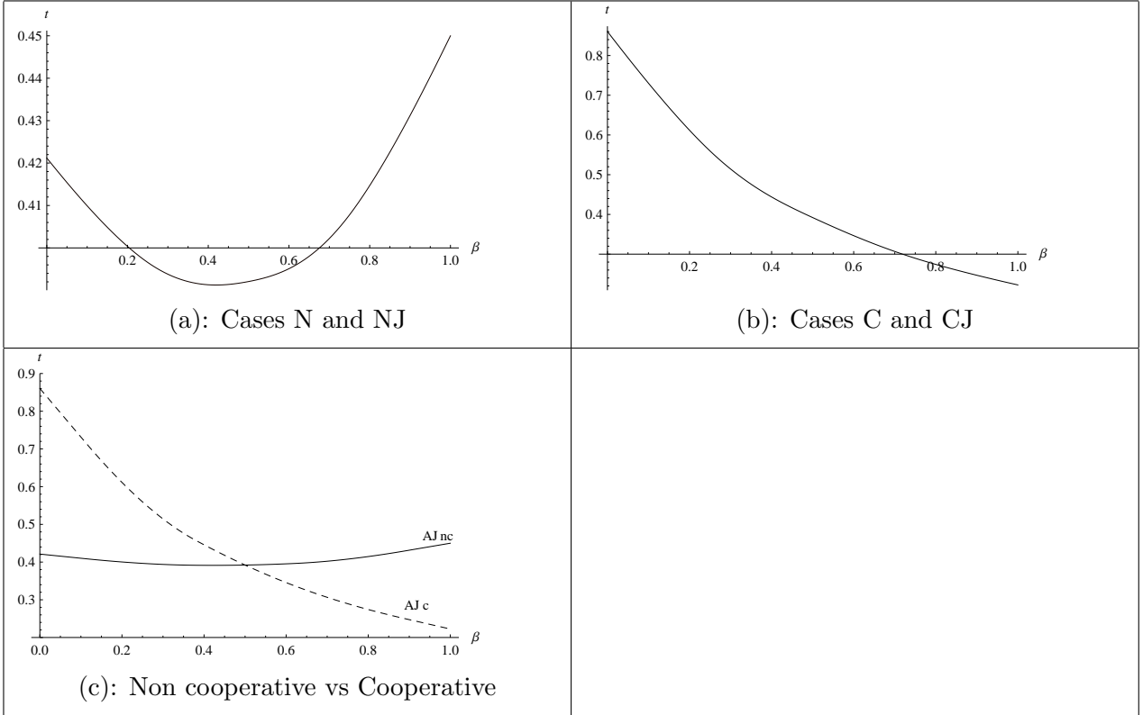
Figure 1: Optimal emissions tax - AJ Model ( a = 20, e = 0.5, \gamma = 8 )
