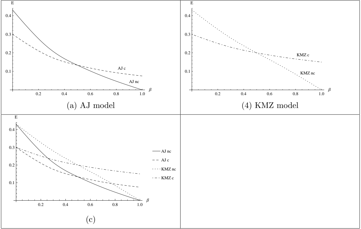
Figure 4: Equilibrium Emissions ( a = 20, e = 0.5, \gamma = 8 )
