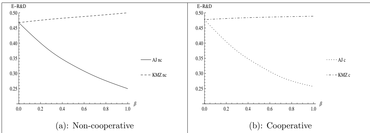
Figure 6: E-R&D - Cooperative vs Non-cooperative ( a = 20, e = 0.5, \gamma = 8 )
