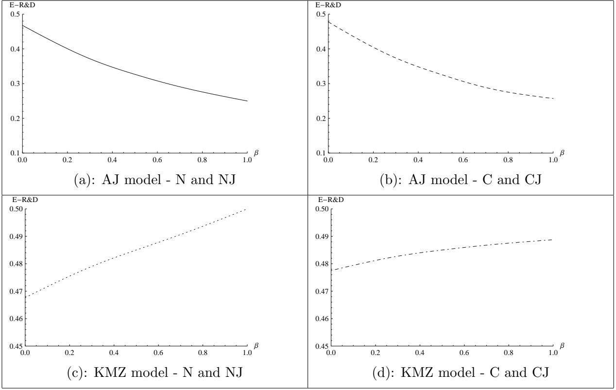
Figure 5: E-R&D (abatement activity) ( a = 20, e = 0.5, \gamma = 8 )
