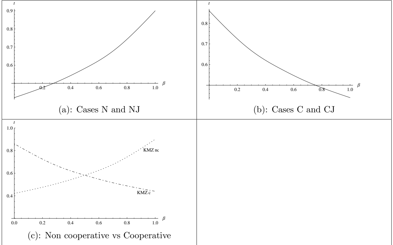
Figure 2: Optimal emissions tax - KMZ Model ( a = 20, e = 0.5, \gamma = 8 )
