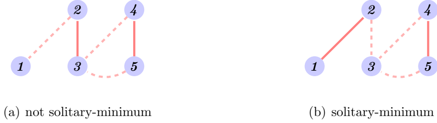
Figure 4: Active-Minimum Matchings
