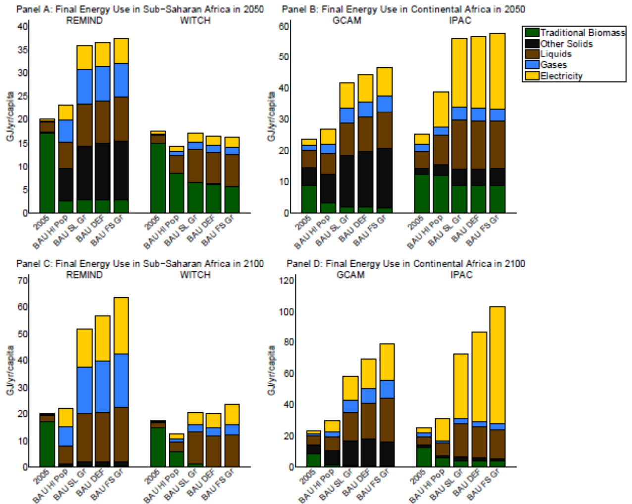
Figure 3 : Final Energy Use per Capita in 2050 and 2100 without Climate Policy
