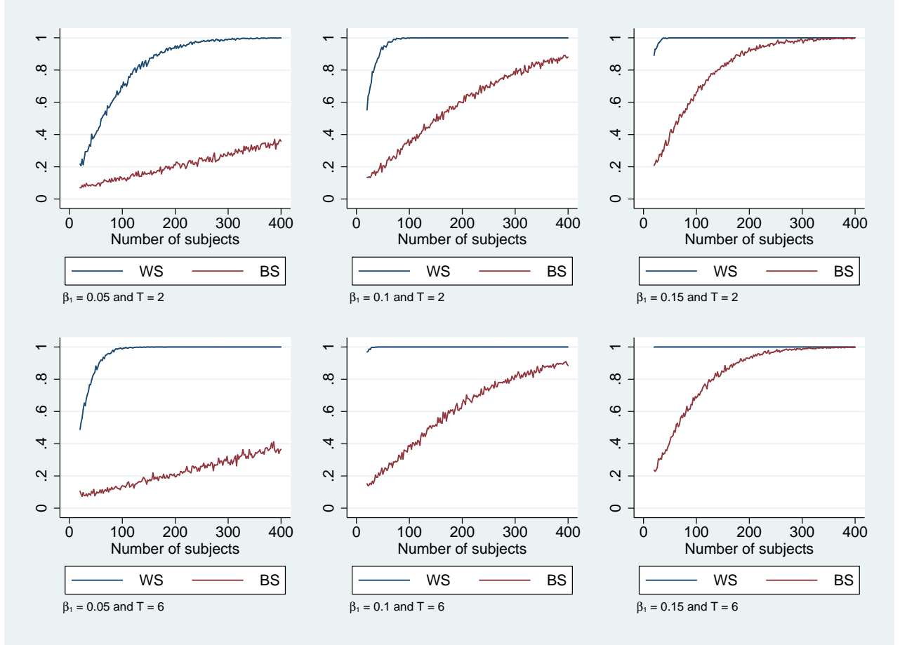
Figure 2: Simulated statistical power of BS and WS designs with T = 2 and T = 6 for the high noise scenario. Simulations based on values \sigma_\mu^2 = 0.09 and \sigma_\epsilon^2 = 0.02 . Results for the BS design are computed by allocating the same number of subjects to control and treatment conditions. Results for the WS design are computed by assigning subjects to the same number of control and treatment periods.
