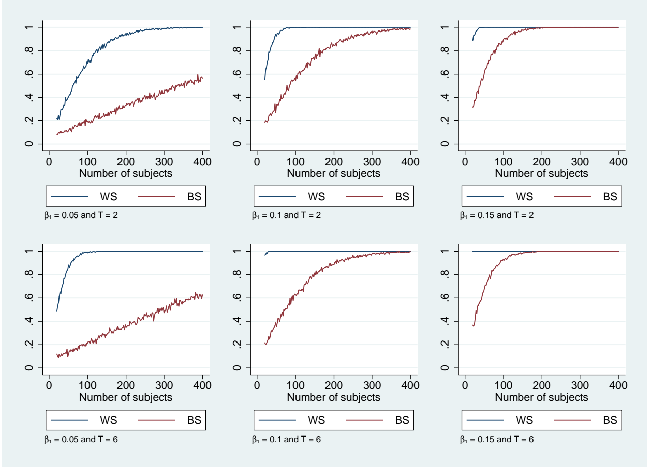
Figure 1: Simulated statistical power of BS and WS designs with T = 2 and T = 6 for the low noise scenario. Simulations based on values \sigma_\mu^2 = 0.045 and \sigma_\epsilon^2 = 0.02 . Results for the BS design are computed by allocating the same number of subjects to control and treatment conditions. Results for the WS design are computed by assigning subjects to the same number of control and treatment periods.
