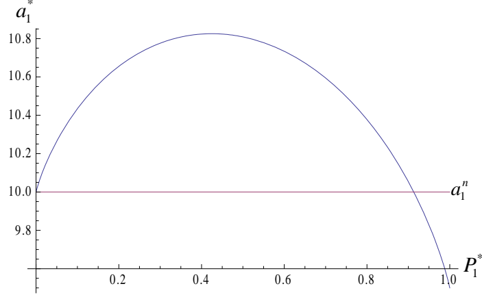
Figure 1: Equilibrium relation between agent 1's effort level a_1^* and his winning probability P_1^* . W(a) = 10 - .5a for a < 18 and W(a) = 1 for a \geq 18 , m_2 = 1 , h_1 = h_2 = 2 , h_\varepsilon = 1 , S_j(a) - c_j(a) = 10a - \frac{a^2}{2} for j = 1, 2 .
