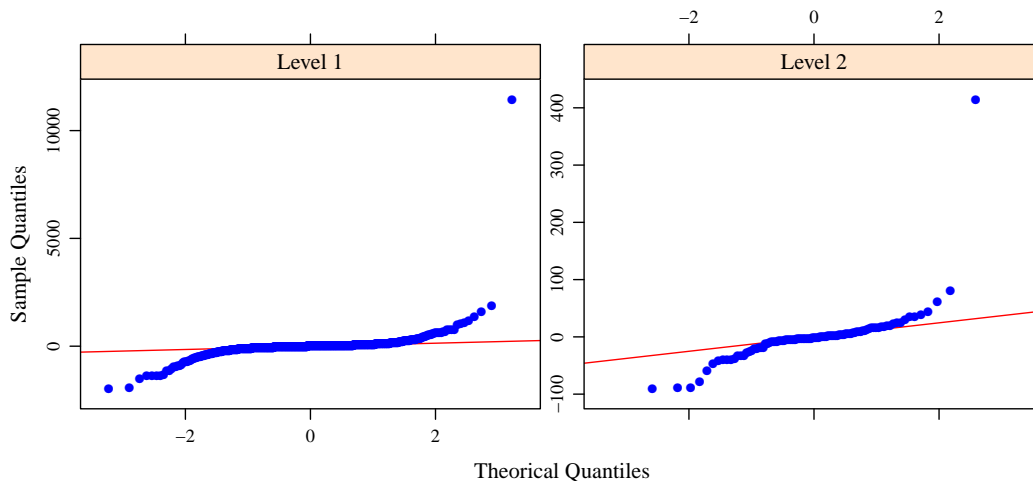
Figure 2: Normal probability plots of level 1 (left) and level 2 (right) residuals.
