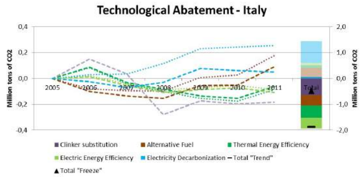
Figure 27: Technological abatement in Italy.
