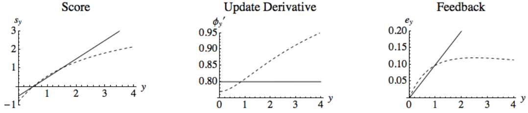
Figure 2: Score function s_y (left), derivative of update function \phi'_y (center), and feedback effect e_y(f_t, y_t; \theta) (right) for thin-tailed GAS model (solid) with \lambda_2 \rightarrow \infty and fat tailed \lambda_2 = 5 GAS model (dashed) with \lambda_1 = 1 , \alpha = 0.1 and \beta = 0.8 .
