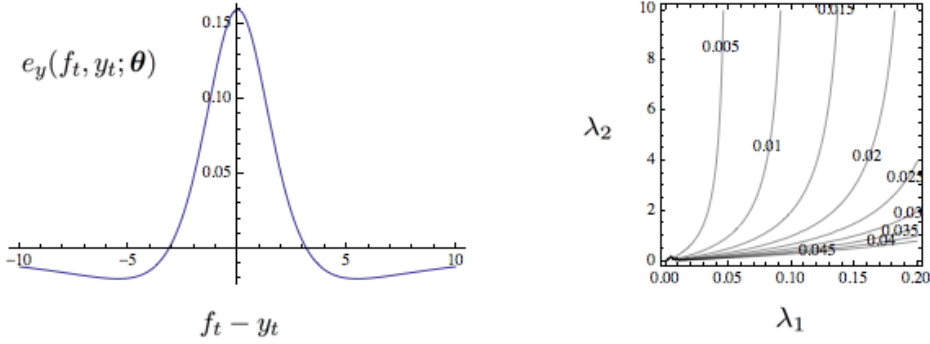
Figure 1: Value of feedback term e_y(f_t, y_t; \theta) (left) as function of f_t - y_t for \alpha = 0.1 , \lambda_1 = 0.5 and \lambda_2 = 5 and contour plot (right) of maximum feedback value in equation (29) as function of \lambda_1 and \lambda_2 .
