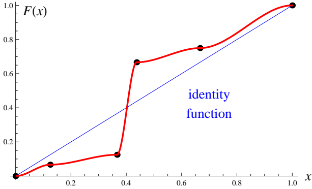
Figure 1: Example 2A: function F generating a monotone (and eventually strongly monotone) \mathbf{F} with an asymptotically stable two-periodic point
