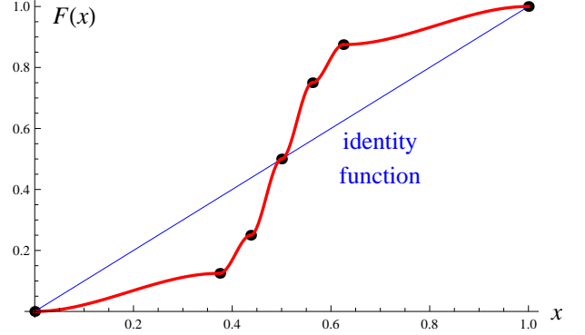
Figure 2: Example 2B: function F generating a monotone (and eventually strongly monotone) \mathbf{F} with an asymptotically stable asymmetric steady state
