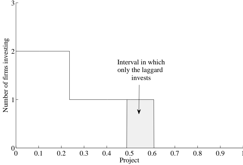
Figure 6: Asymmetric firms.
