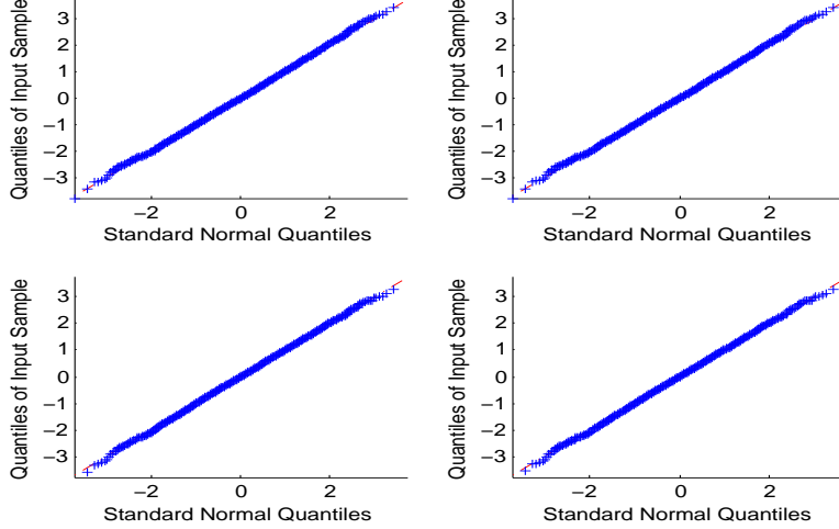
Figure 7.2: QQ-Plot for t tests \hat{t}_j for j = 1, 2 for a linear functional (first row) and a nonlinear functional (second row) of NPIV, with q^{k(n)} = Pol(4) and p^{J_n} = Pol(16) .
