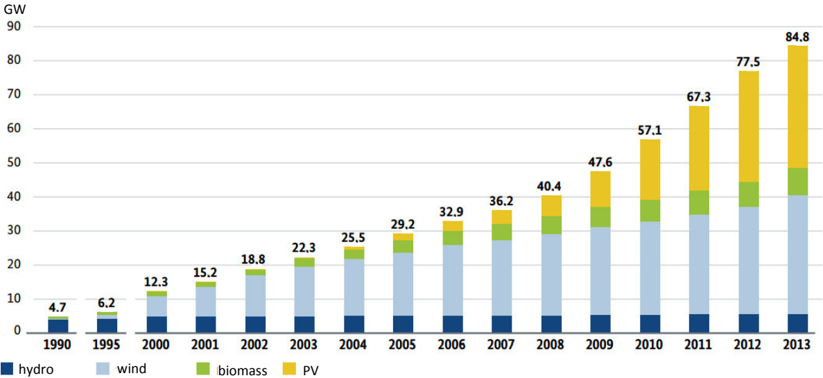
Figure 1: Development of installed RES capacity in Germany [BMWi 2014a]
