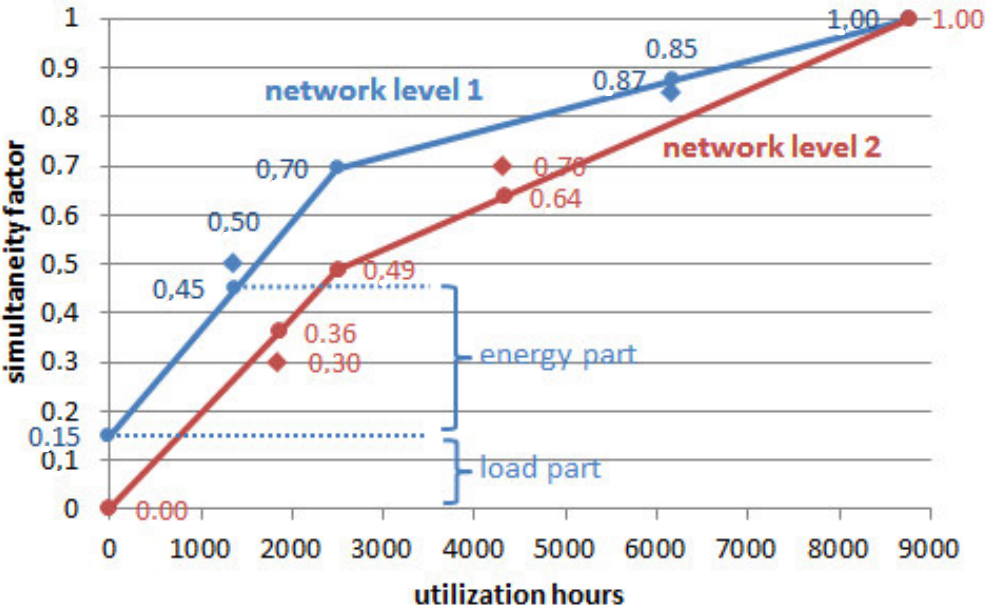
Figure 12: Example simultaneity functions for two subsequent levels with three customers
