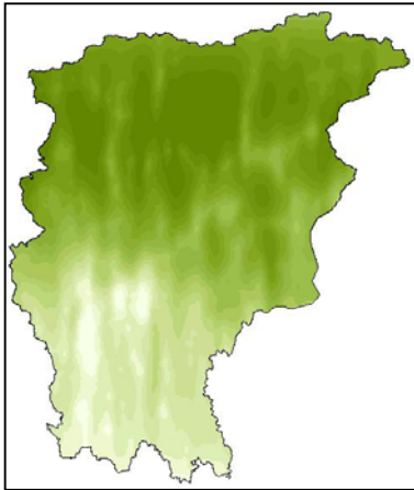
Figure 3 \beta 0.0075
