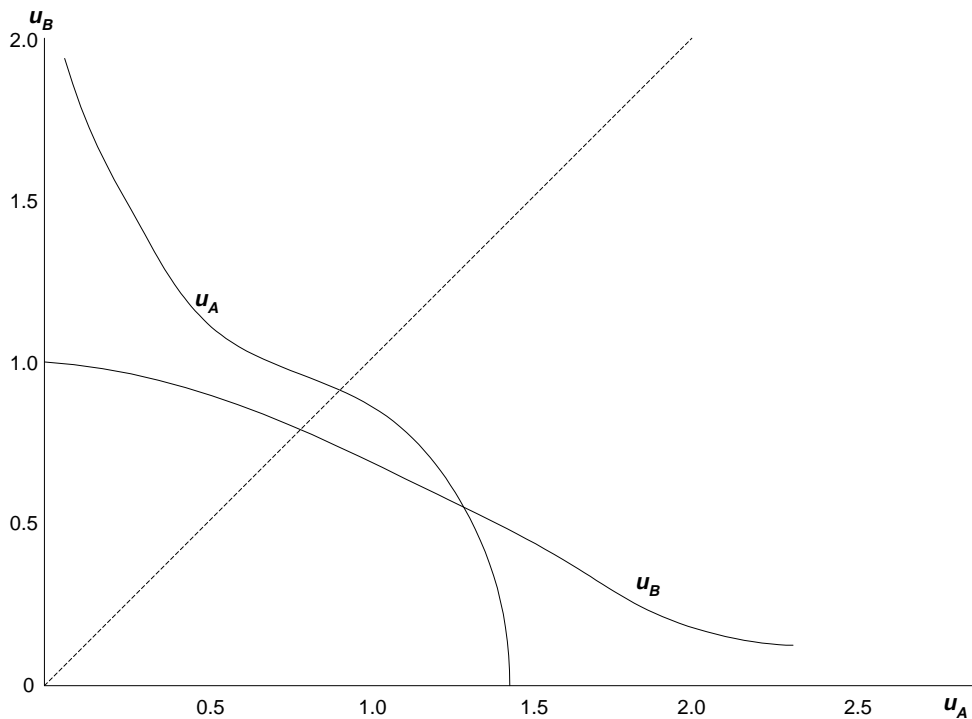
Figure 1: Existence of a Majority Equilibrium
