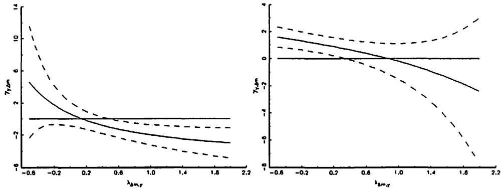
(b) 95% Confidence Intervals for \gamma_{y,\Delta m} as a function of \lambda_{y,\Delta m}
