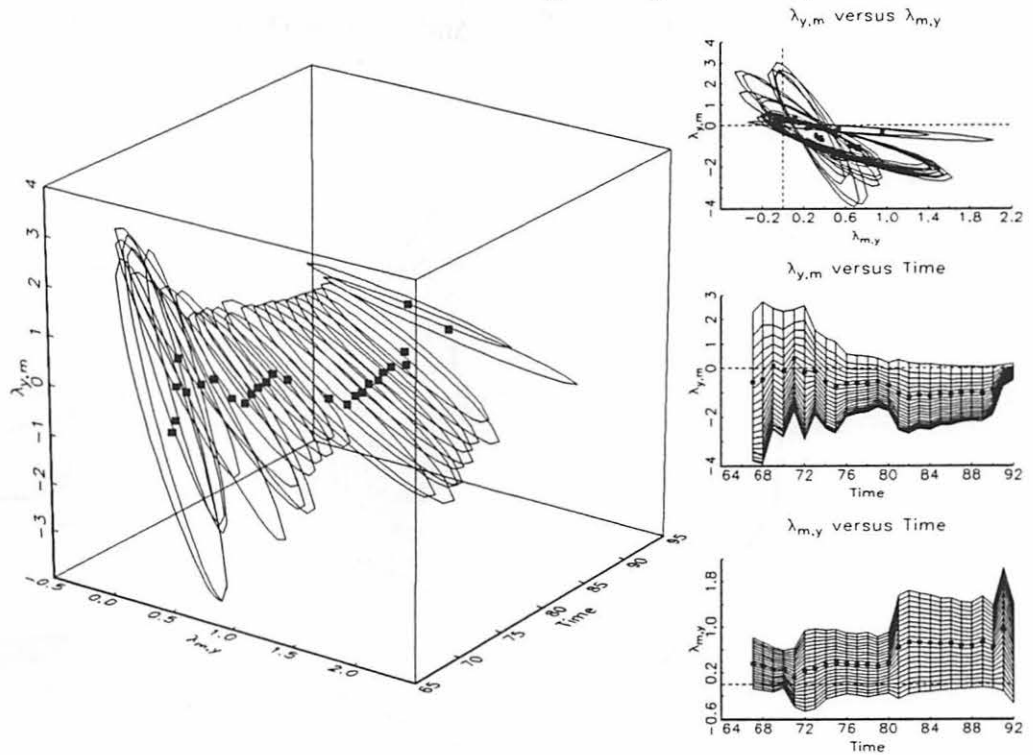
(d) Confidence Ellipses for \lambda_{m,y} and \lambda_{y,m} when \gamma_{y,m} = 0
