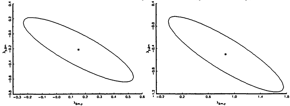
(d) 95 % Confidence Ellipses for \lambda_{y,\Delta m} and \lambda_{\Delta m,y} imposing \gamma_{y,\Delta m}=0
