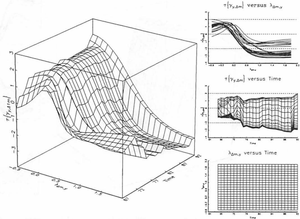
(b) T-test for \gamma_{y,\Delta m} \neq 0 as a function of \lambda_{y,\Delta m} and time
