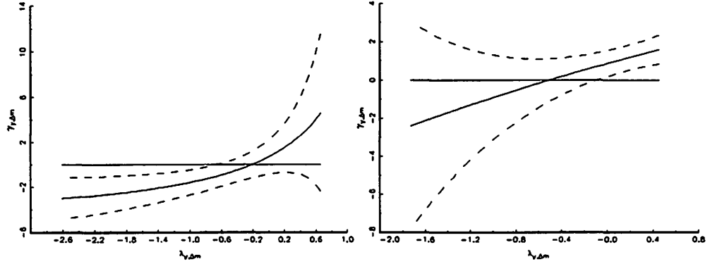
(c) 95% Confidence Intervals for \gamma_{y,\Delta m} as a function of \gamma_{\Delta m,y}
