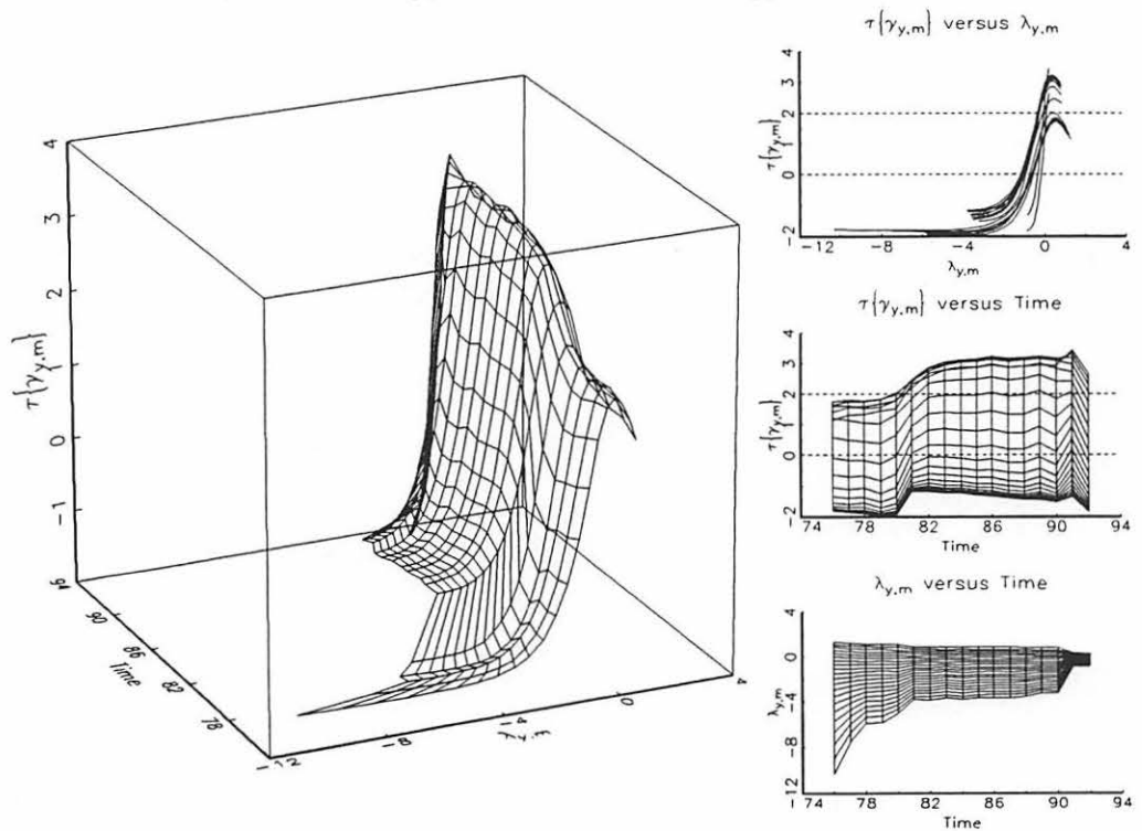
(b) T-test for \gamma_{y,m} \neq 0 as a function of \lambda_{y,m} and time
