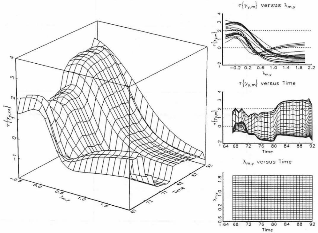
(a) T-test for \gamma_{y,m} \neq 0 as a function of \lambda_{m,y} and time
