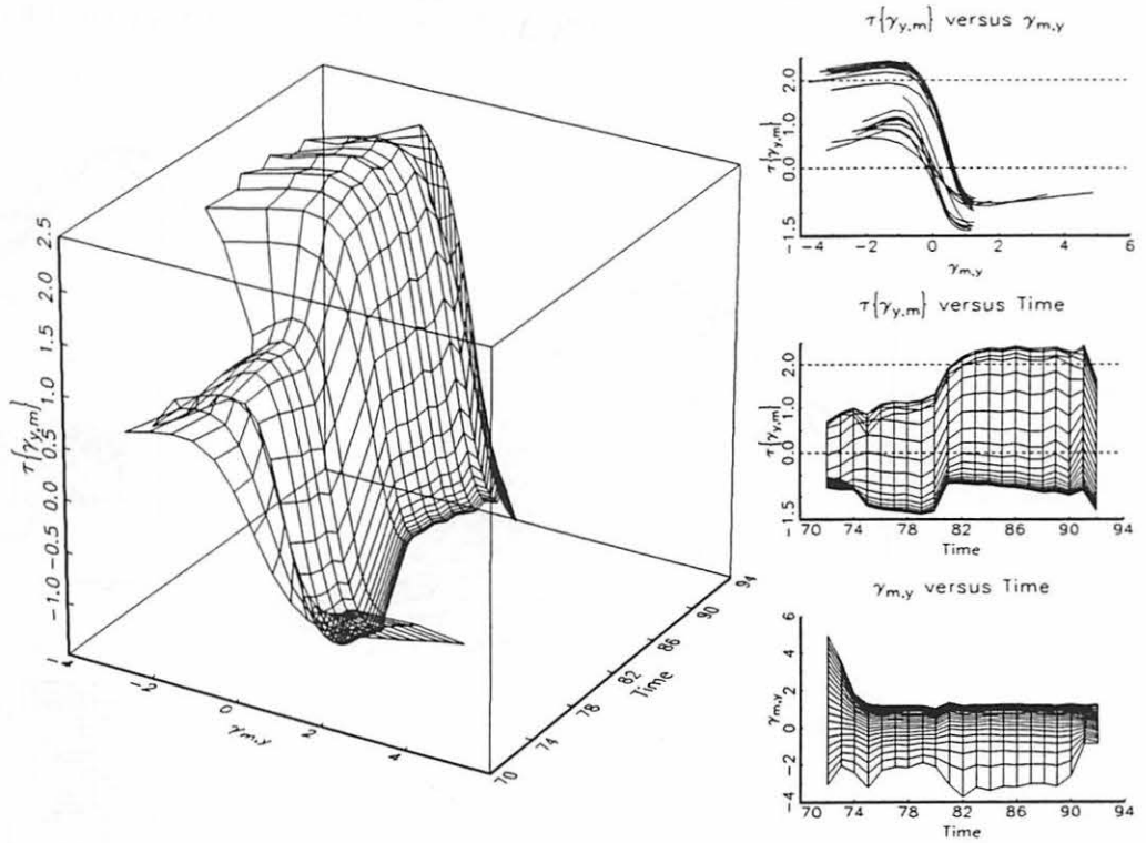
(c) T-test for \gamma_{y,m} \neq 0 as a function of \gamma_{m,y} and time
