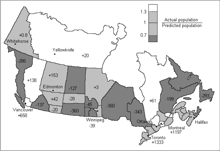
Figure 4: Projected vs. actual population according to the main model, Canada 1991. (Numbers show the absolute difference between projected and actual population, in thousands).
