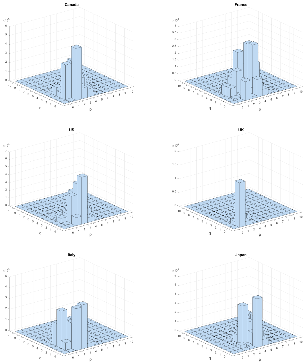
Figure 6: Posteriors for model indicators
