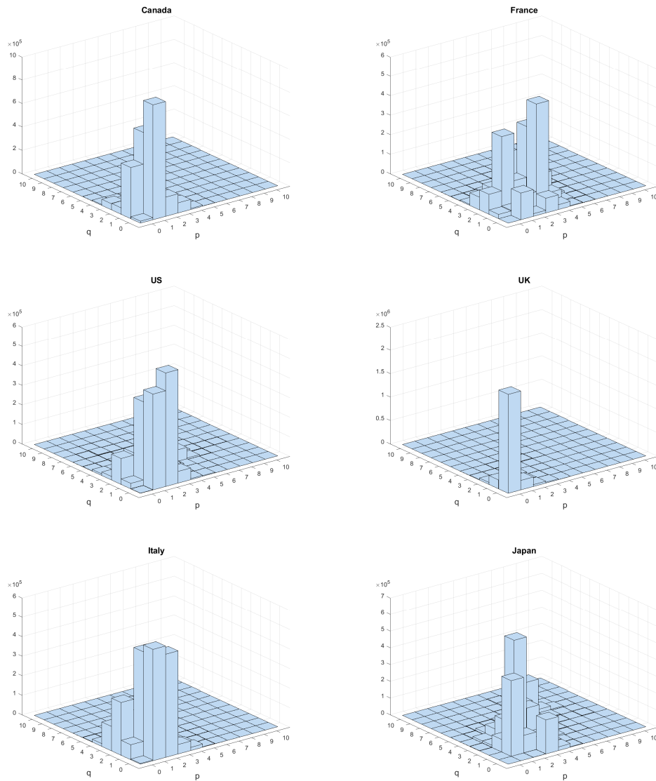
Figure 2: Posteriors for model indicators
