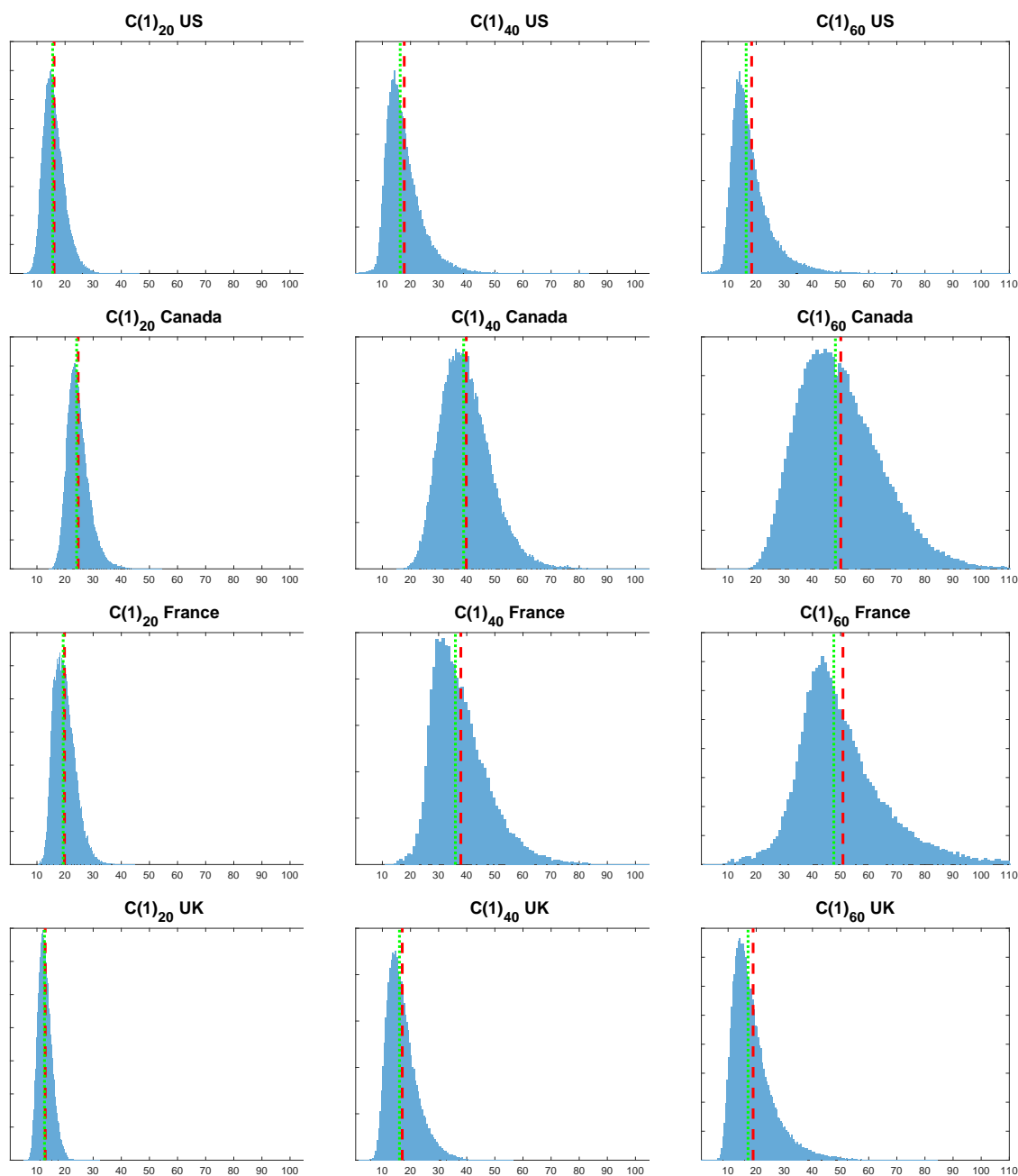
Figure 8: C(1) : Mean: Dashed line; Median: Dotted line
