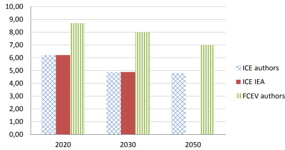
Figure 4: Fuel consumption ICE (1/100km) FCEV (kg/10km)
