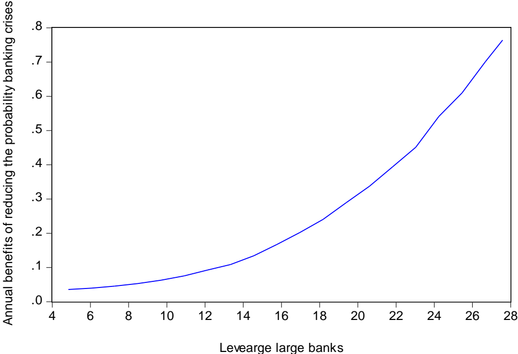
Exhibit 15: Expected annual GDP benefits and trend leverage of large banks.
