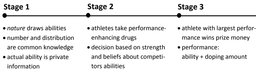
Figure 1: The information structure of the contest
