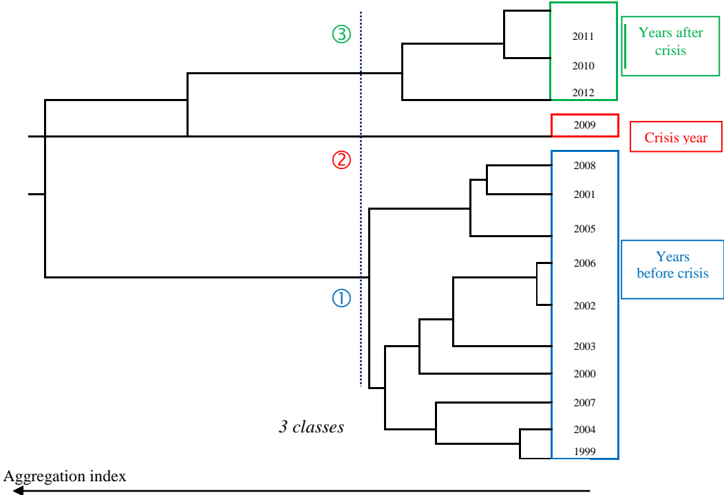
Figure 3: Cluster dendrogram of years over the period 1999 to 2012 according to the means of the economic and entrepreneurial activity variables of the 26 OECD countries 13
