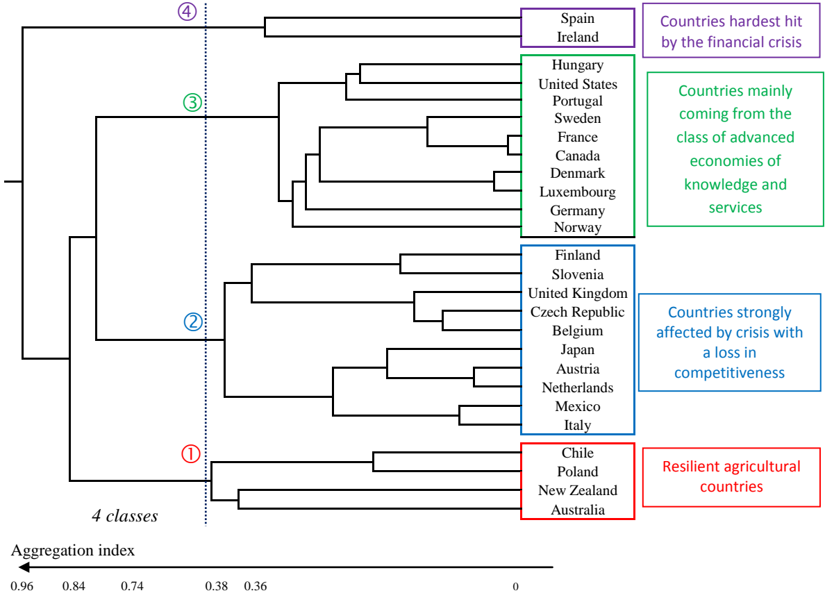
Figure 6: Hierarchical tree in 2009 for the 26 OECD countries
