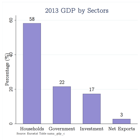
Figure 1.3: By sectors
