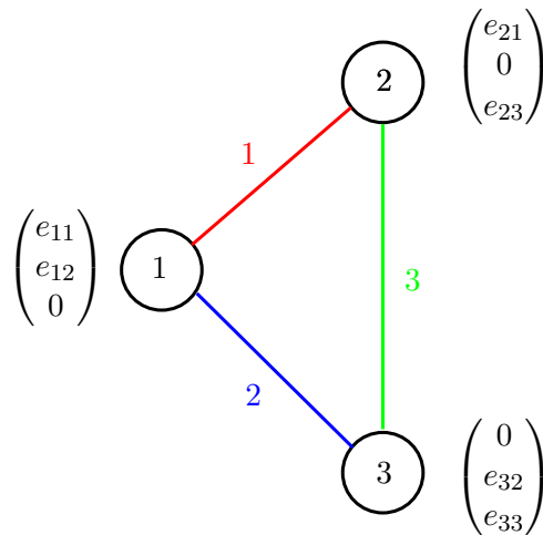
Figure 5: The network analyzed in Example 3. The effort levels of the individual agents for each project they are involved in are indicated next to the nodes.
