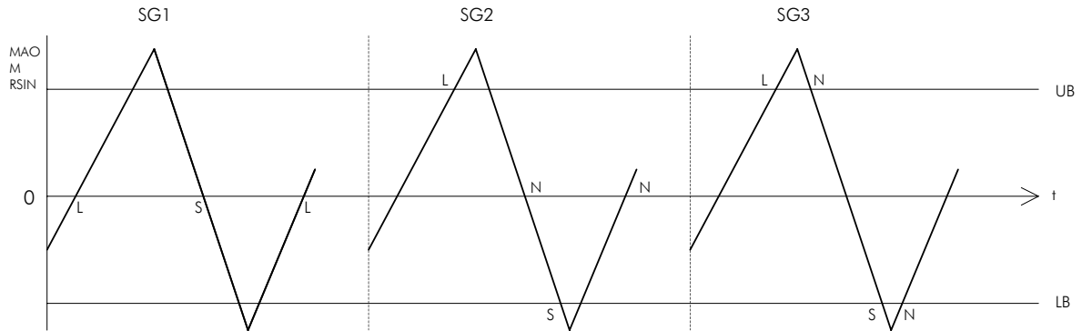
Figure 1: Signal generation of technical trading systems
