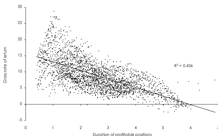
Figure 8: Duration of profitable positions and the performance of 2,580 trading systems S & P 500 futures market, 30-minutes-data, 1983-2007
