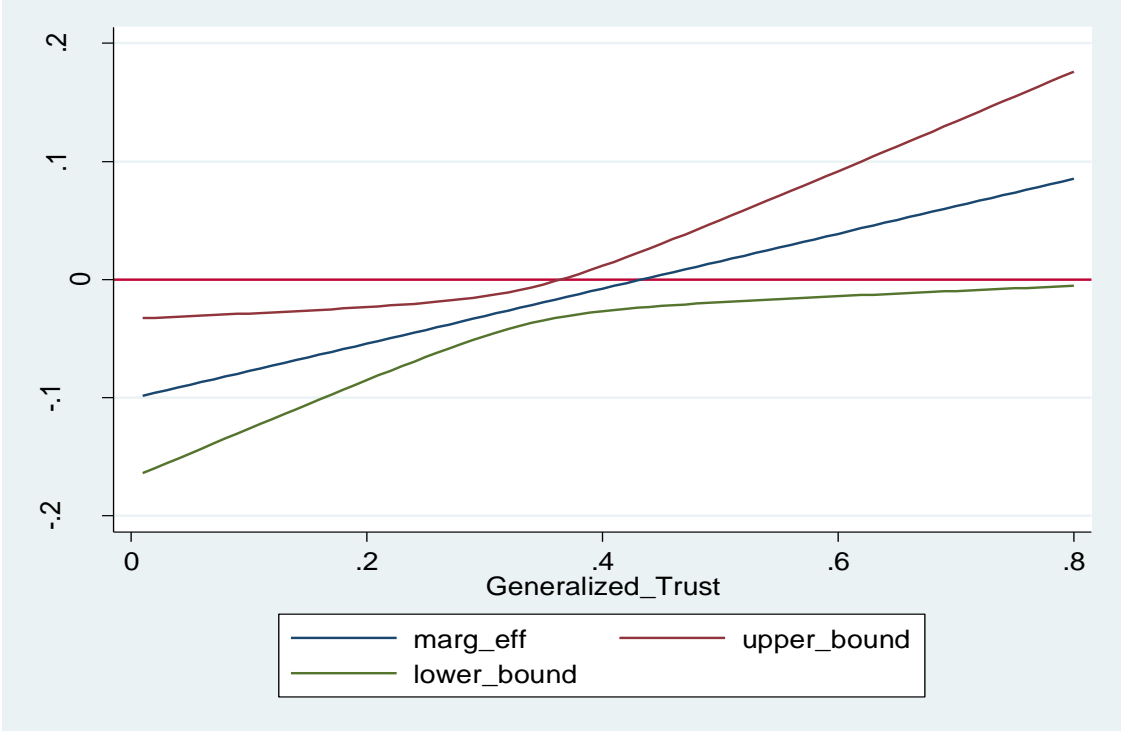
Figure 2: Total marginal effects of num_coal_(it) at various levels of trust_av_(it)
