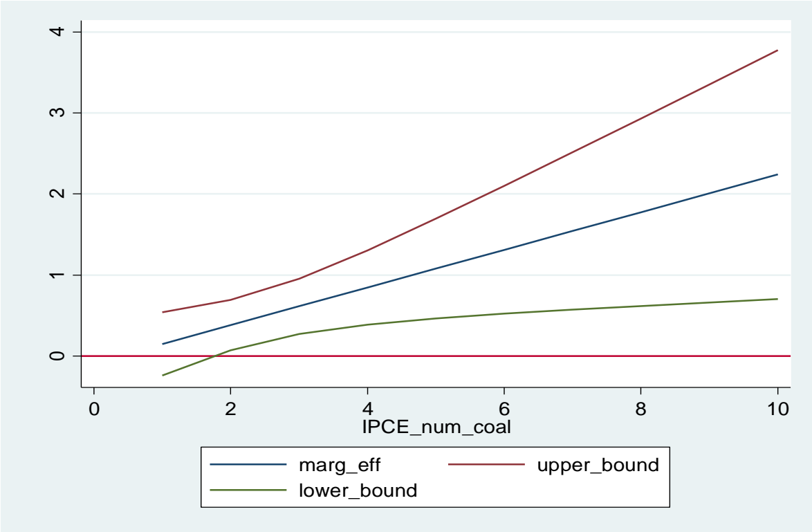
Figure 4: Total marginal effects of trust_av_(it) at various levels of num_coal_(it)
