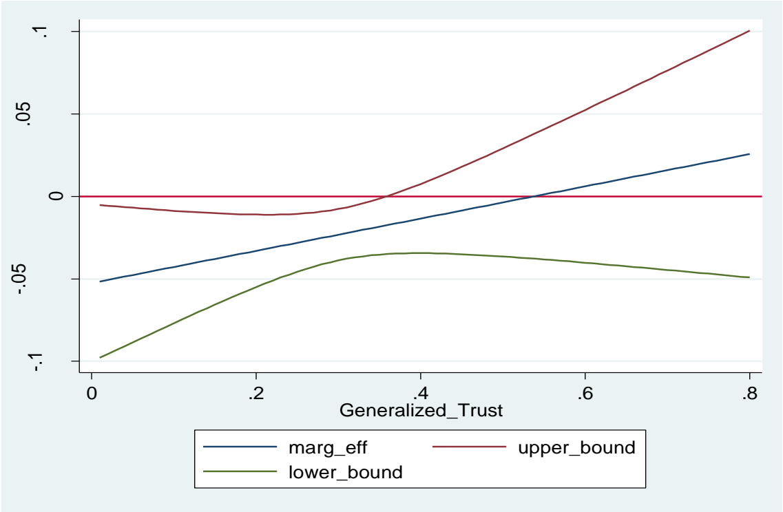
Figure 2: Total marginal effects of num_coal_(it) at various levels of trust_av_(it)
