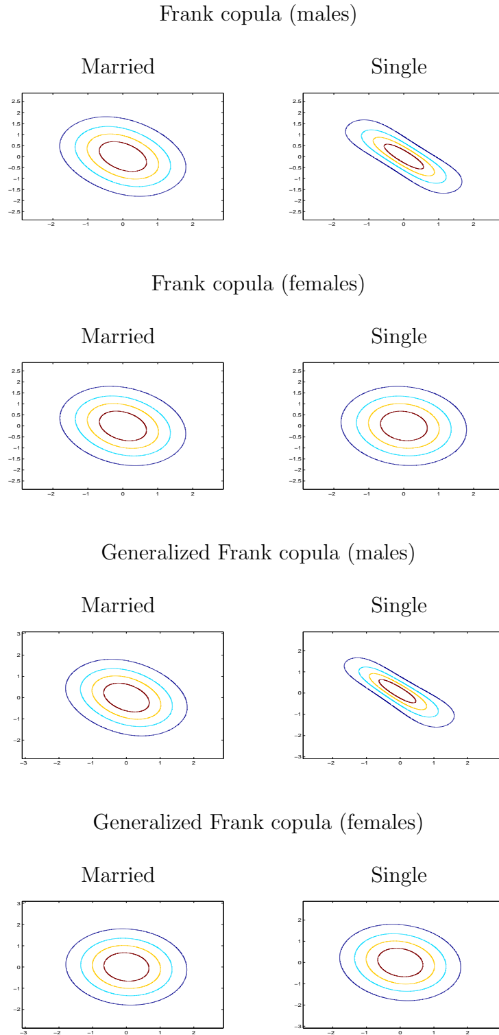
Figure 4: Contour plots of the copula
