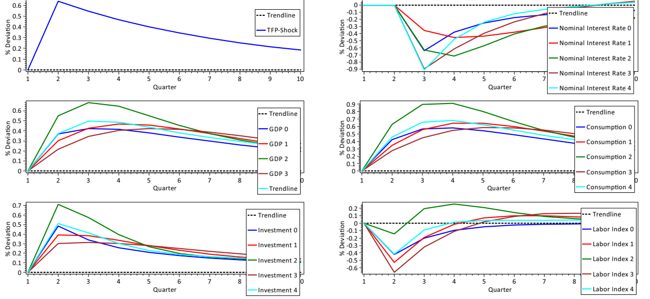
Figure 4.1: Impulse responses 1
