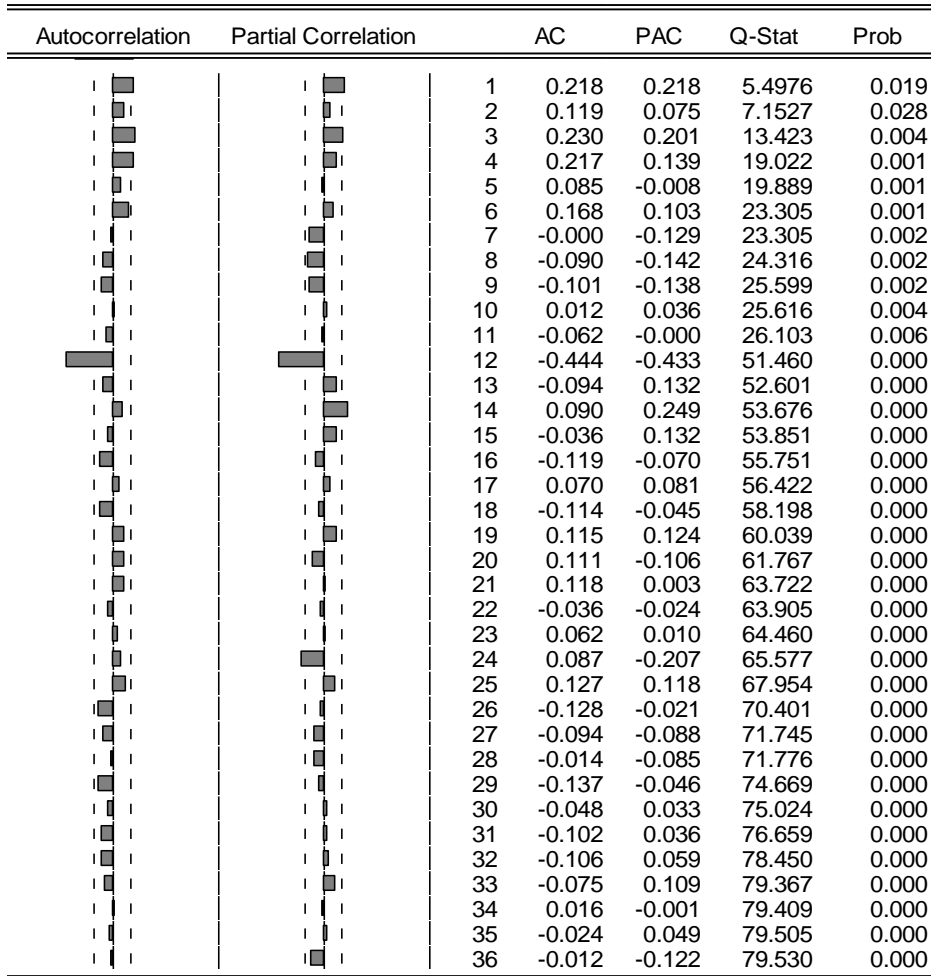
Fig 5: ACF and PACF Plot of \Delta^{12}dlog(ER_t)
