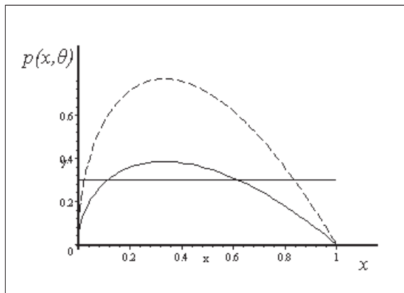
Fig. 1: Demand shift with FSD shock.
