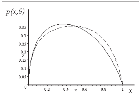
Fig. 2: Demand shift with single crossing SSD shock.
