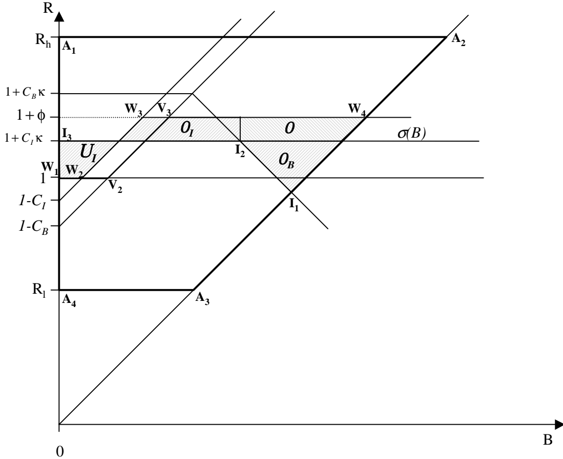
Figure 4: Over- and under- investment regions for decentralised financial conglomerates.
