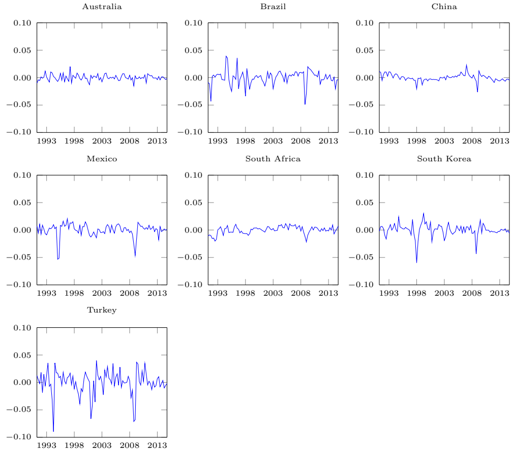
Figure 2: Detrended annualized quarterly GDP growth of the OIC
