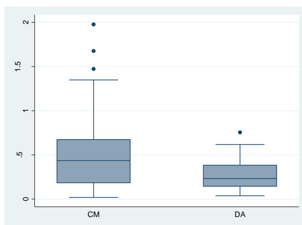
Figure 3: Efficient Price Smith's Alpha
