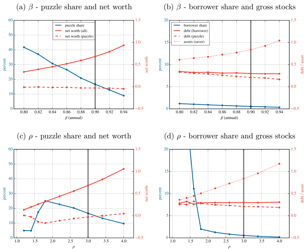
Figure 6.2: Alternative Preferences
