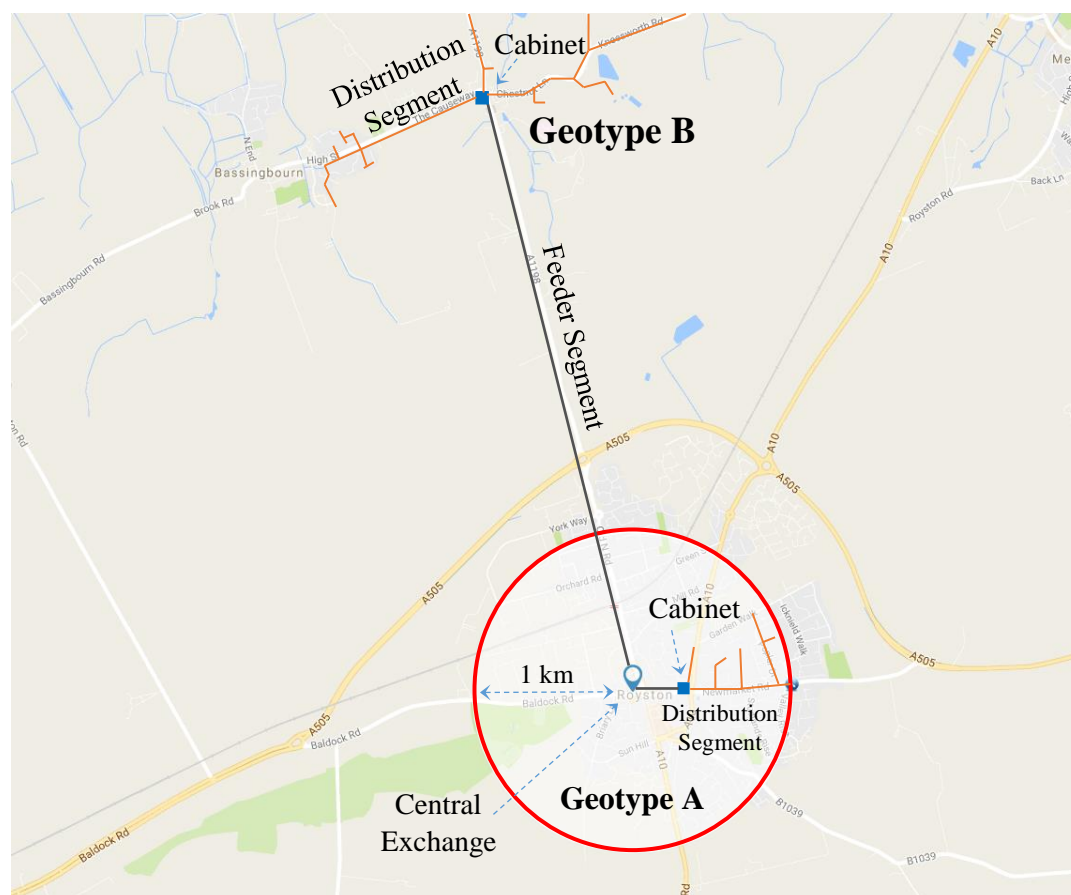
Figure 2 Examples of network elements in Geotype A and Geotype B emanating from the central telephone exchange in Royston, Hertfordshire, UK
