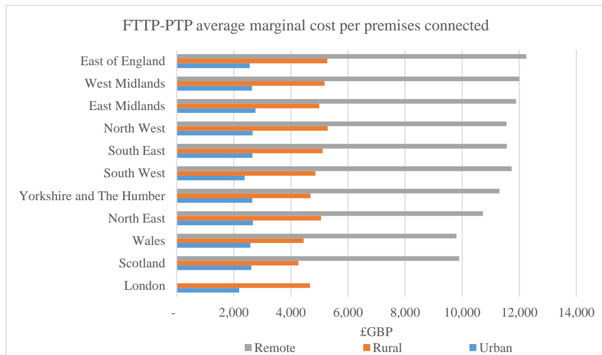
Figure 4 FTTP-PTP average marginal cost per premises connected by region and geotype
