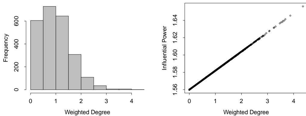
Figure 4: The left panel: the histogram of the weighted degrees; the right panel: the influential power against weighted degrees.
