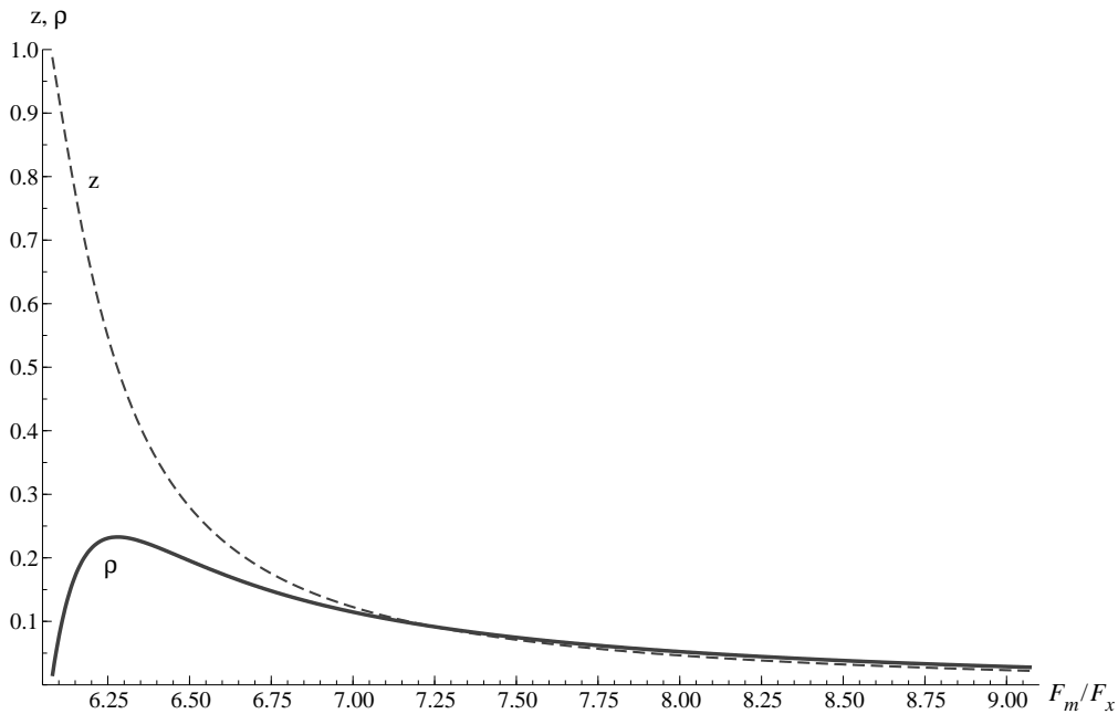
Figure 4: The permissible parameter range identified by calibration
