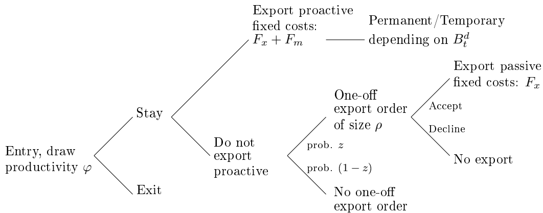
Figure 3: Schematic illustration of the model
