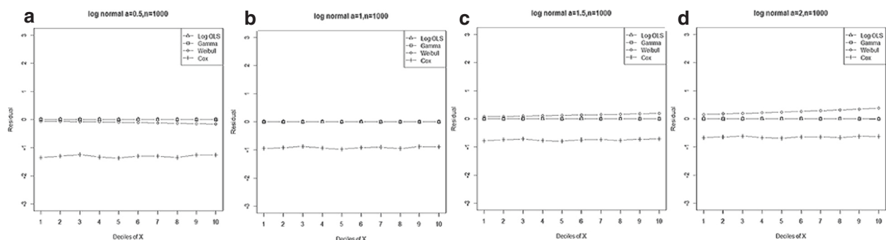
Figure 13 Mean residual from different estimators across deciles of 'X' for log-normal data ( n=1000 ) with variance a: 0.5, b: 1.0, c: 1.5, d: 2.0.
