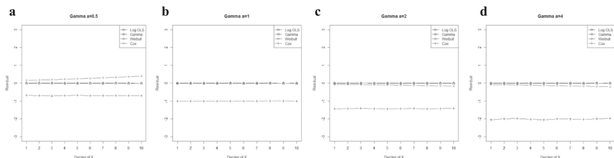
Figure 14 Mean residual from different estimators across deciles of 'X' for Gamma data ( n=1000 ) with shape parameter a: 0.5, b: 1, c: 2, d: 4.
