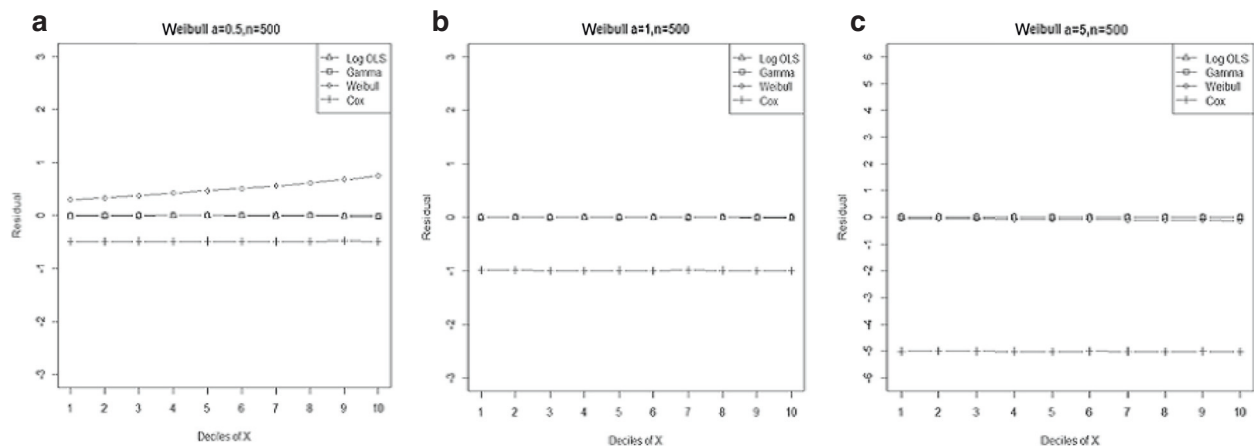
Figure 12 Mean residual from different estimators across deciles of 'X' for Weibull data ( n=500 ) with shape parameter a: 0.5, b: 1, c: 5.
