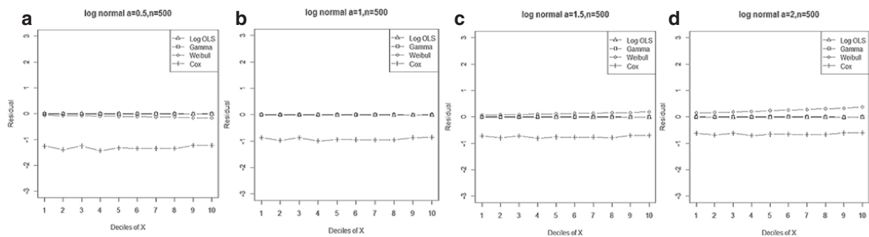
Figure 10 Mean residual from different estimators across deciles of 'X' for log-normal data (n=500) with variance a: 0.5, b: 1.0, c: 1.5, d: 2.0.
