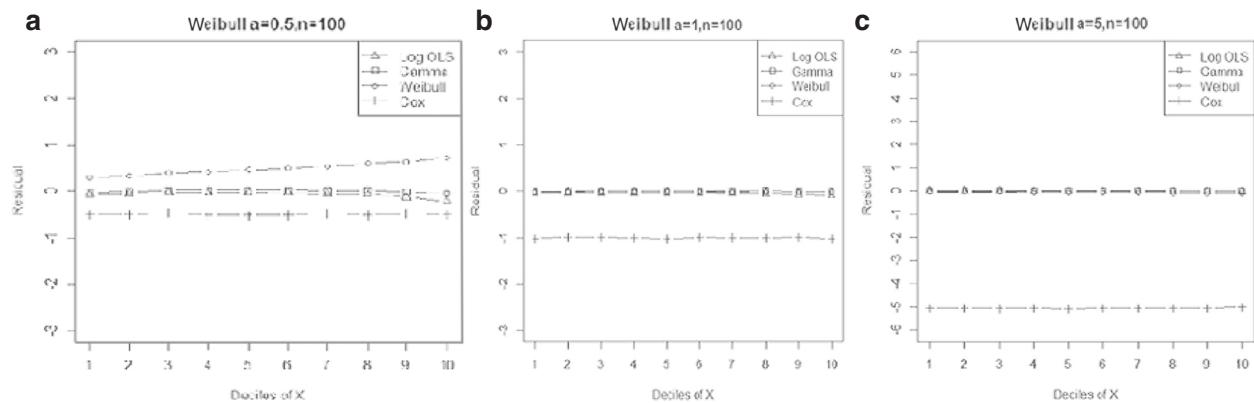
Figure 9 Mean residual from different estimators across deciles of 'X' for Weibull data (n=100) with shape parameter a: 0.5, b: 1, c: 5.
