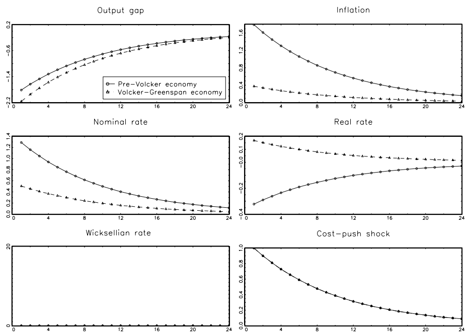
Fig. 4: Impulse responses to unit cost push-shock. Line with circles has \lambda = 0.4 and \phi_{\pi} = 0.8 ; line with triangles has \lambda = 0.05 and \phi_{\pi} = 1.5 . Otherwise baseline parameterization.
