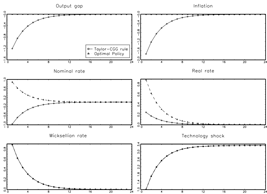
Fig. 5: Impulse responses to unit shock to technology growth. Estimated rule is with circles, optimal policy with triangles.
