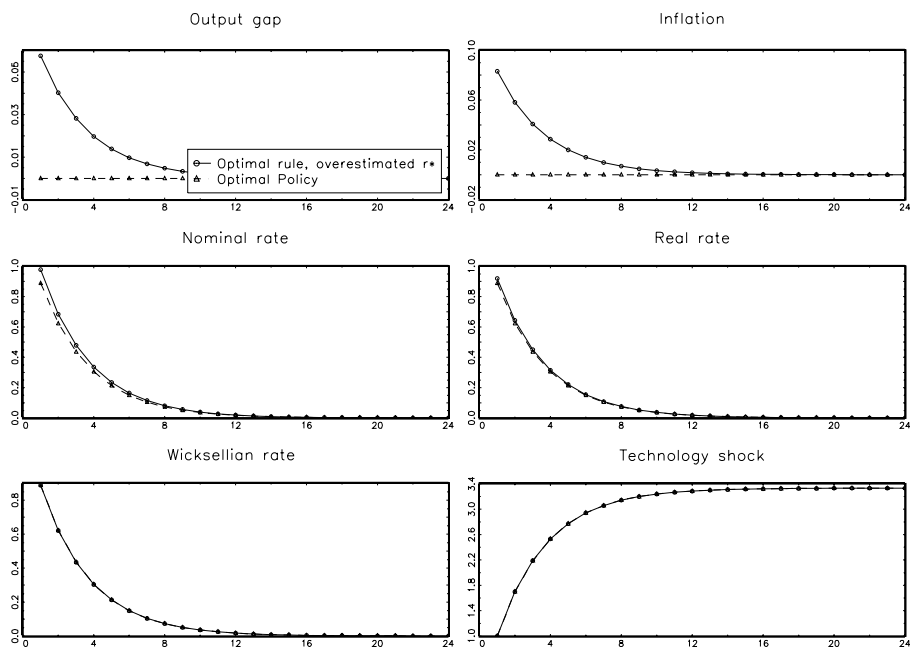
Fig. 6: Estimated responses to unit technology growth shock. In the 'circles' economy, natural rate of interest is systematically overestimated.
