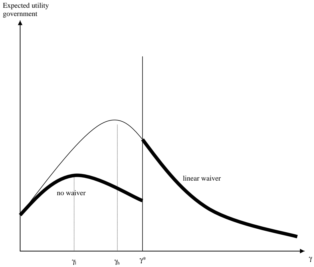
Figure 1: sophisticated scheme enhances reform; optimum is \gamma^*
