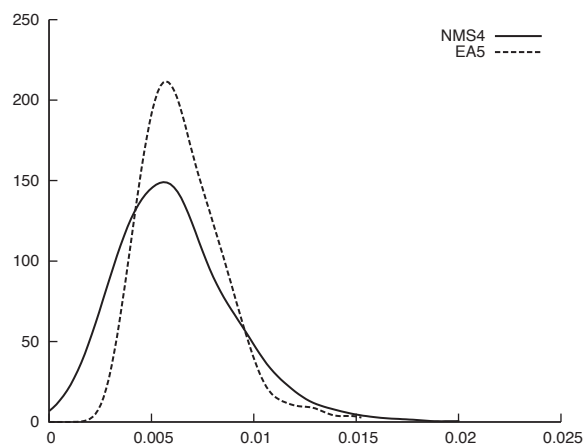
Figure 8: Simulated posterior distribution of \sqrt{\lambda} in the NMS4 panel and in the EA5 panel
