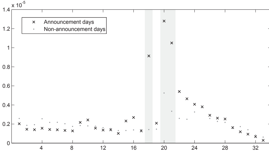
Figure 4: Average intradaily increments in quadratic covariation estimates.
