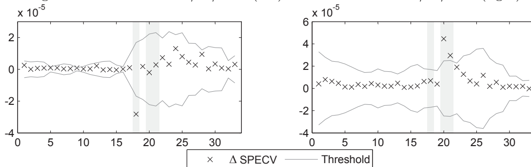
Figure 10: Rotation on 03/07/2002 (left) and level shifts on 10/02/2008 (right).
