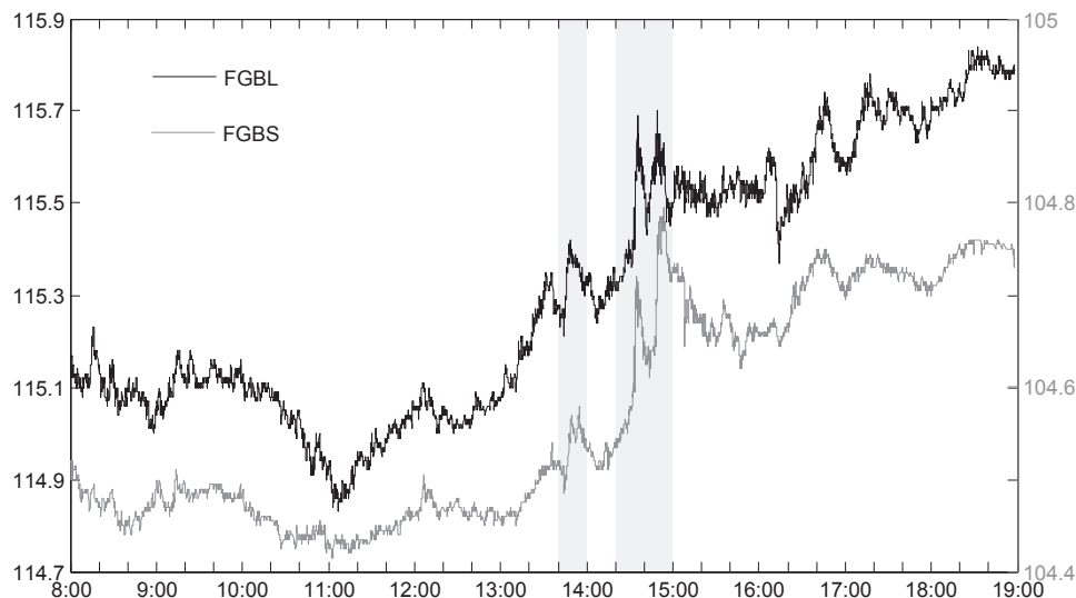
Figure 2: German government bond futures on October, 2. 2008.
