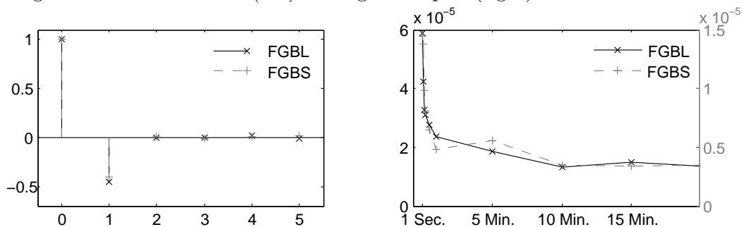
Figure 9: Autocorrelation (left) and signature plot (right) for FGBS and FGBL.
