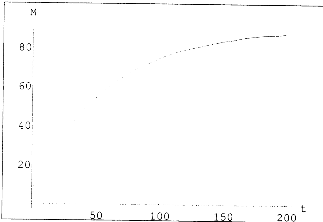
Figure 4: Evolution of \text{CO}_2 concentration at the noncooperative solution
